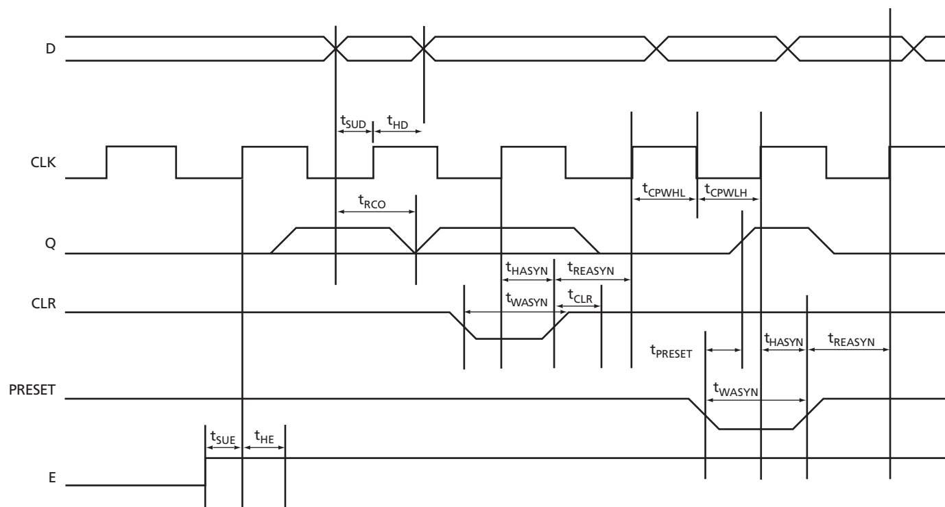
Figure 2-32 • R-Cell Delays
